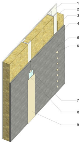
Diagram 1 - typical construction detail with joint filler and mesh tape
