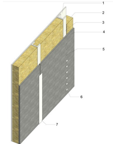
Diagram 2 - typical construction detail with tape
