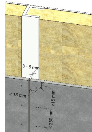
Diagram 3 - typical detail of fixing layout
